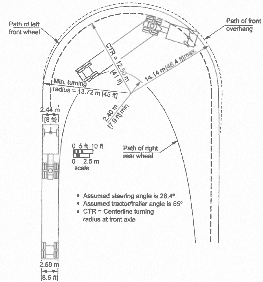
Exhibit 2-15. Minimum Turning Path for Interstate Semitrailer (WB-19 [WB-62]) Design Vehicle
