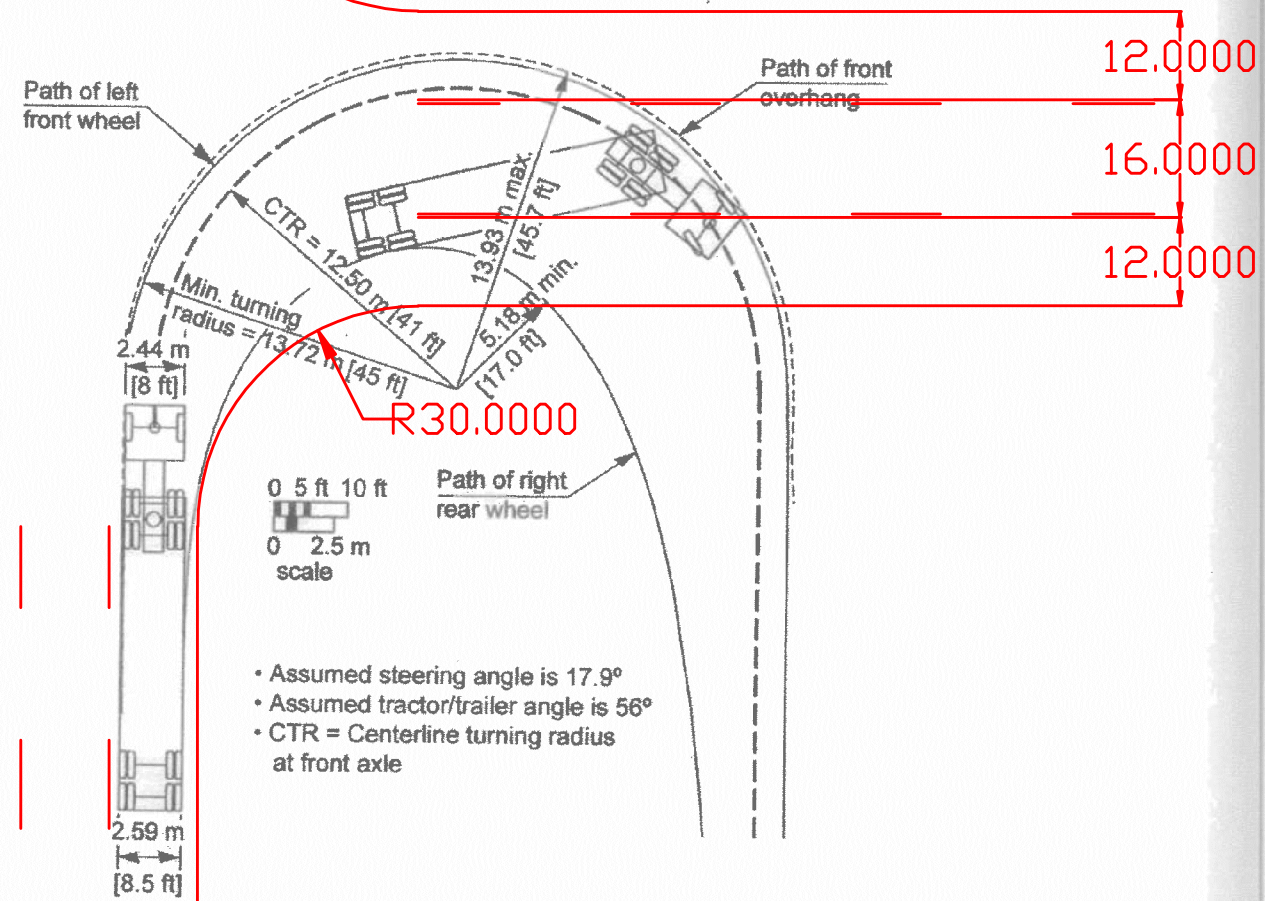
Exhibit 2-14. Minimum Turning Path for Intermediate Semitrailer (WB-15 [WB-50]) Design Vehicle
